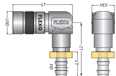
Push to connect hose tail socket 90°
