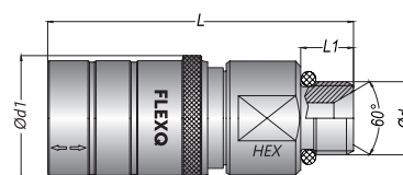
Cone 60°
