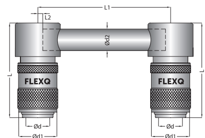
Bridge
