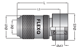
Diverting socket
